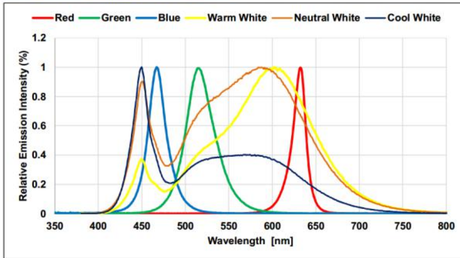
Fig 1. Color Spectrum (光谱图), Ta = 25°C, RH60%
